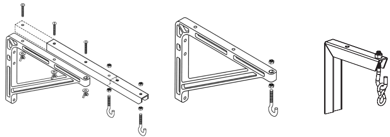
No. 23 Adjustable Wall Bracket Screen can be extended 10", 14", 15 3/4", 18 1/4", 20" or 24" from wall by wing nut and bolt adjustment.
